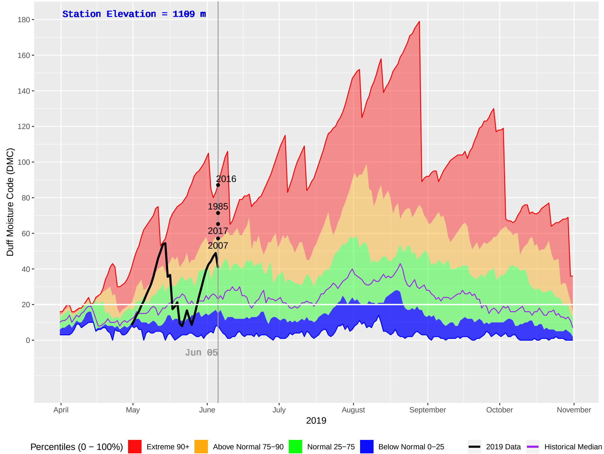
MOOSE LAKE (165) : Historical (1980–2018), Current (2019) Daily Duff Moisture Code (DMC)
