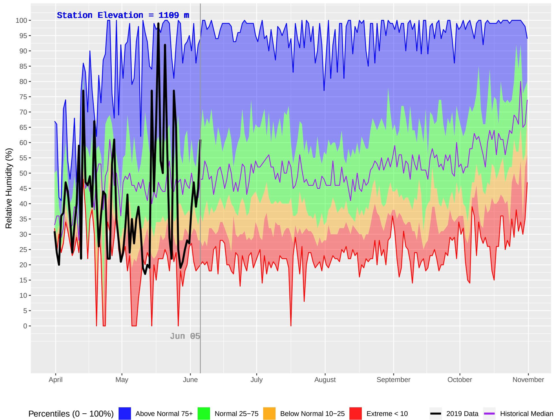
MOOSE LAKE (165) : Historical (1980–2018) and Current (2019) Daily Relative Humidity
