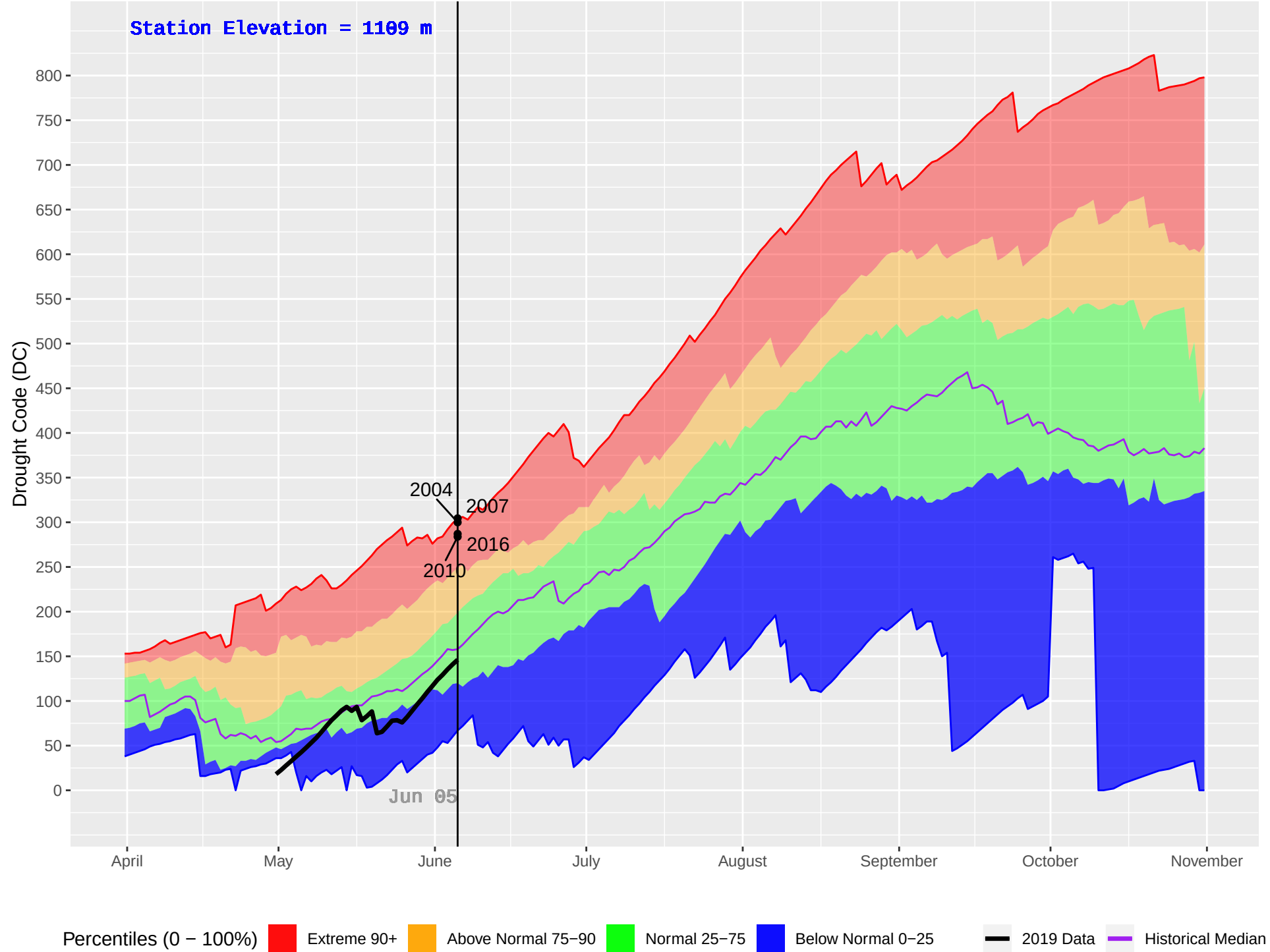
MOOSE LAKE (165) : Historical (1980–2018) and Current (2019) Daily Drought Code (DC)
