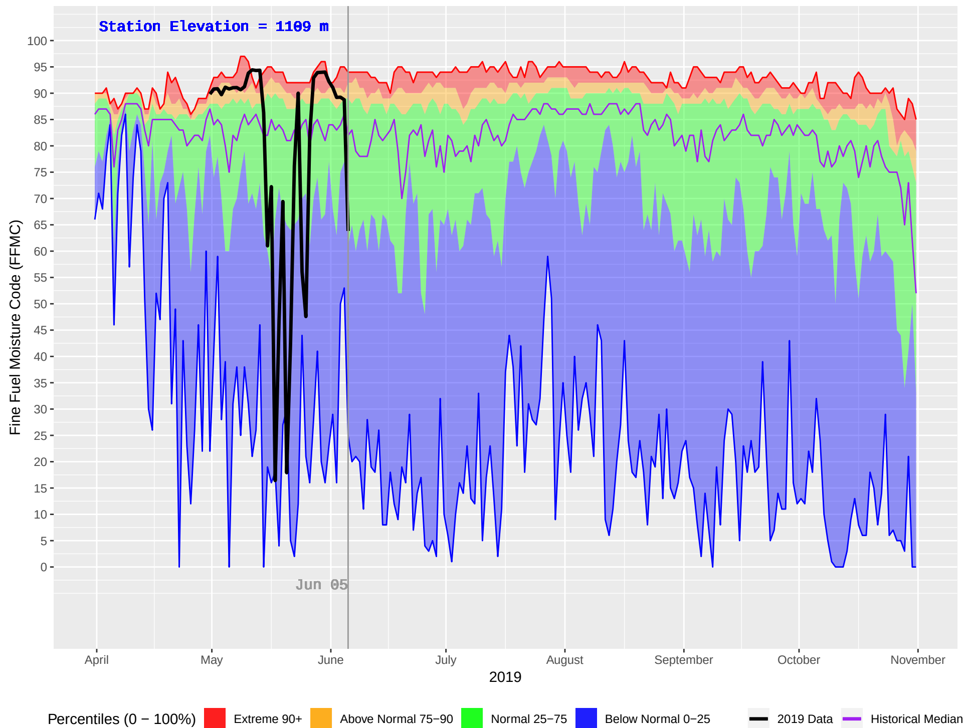
MOOSE LAKE (165) : Historical (1980–2018) and Current (2019) Daily Fine Fuel Moisture Code (FFMC)
