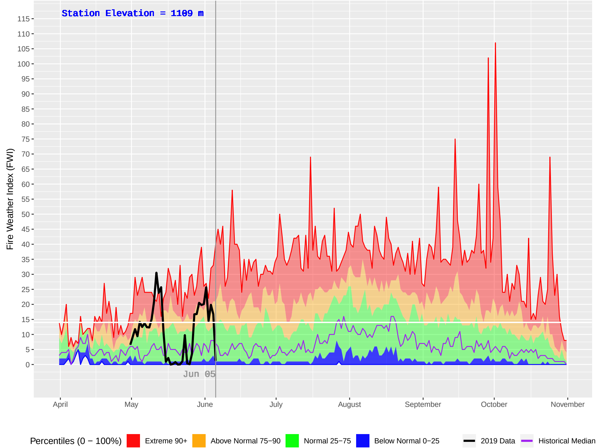
MOOSE LAKE (165) : Historical (1980–2018) and Current (2019) Daily Fire Weather Index (FWI)
