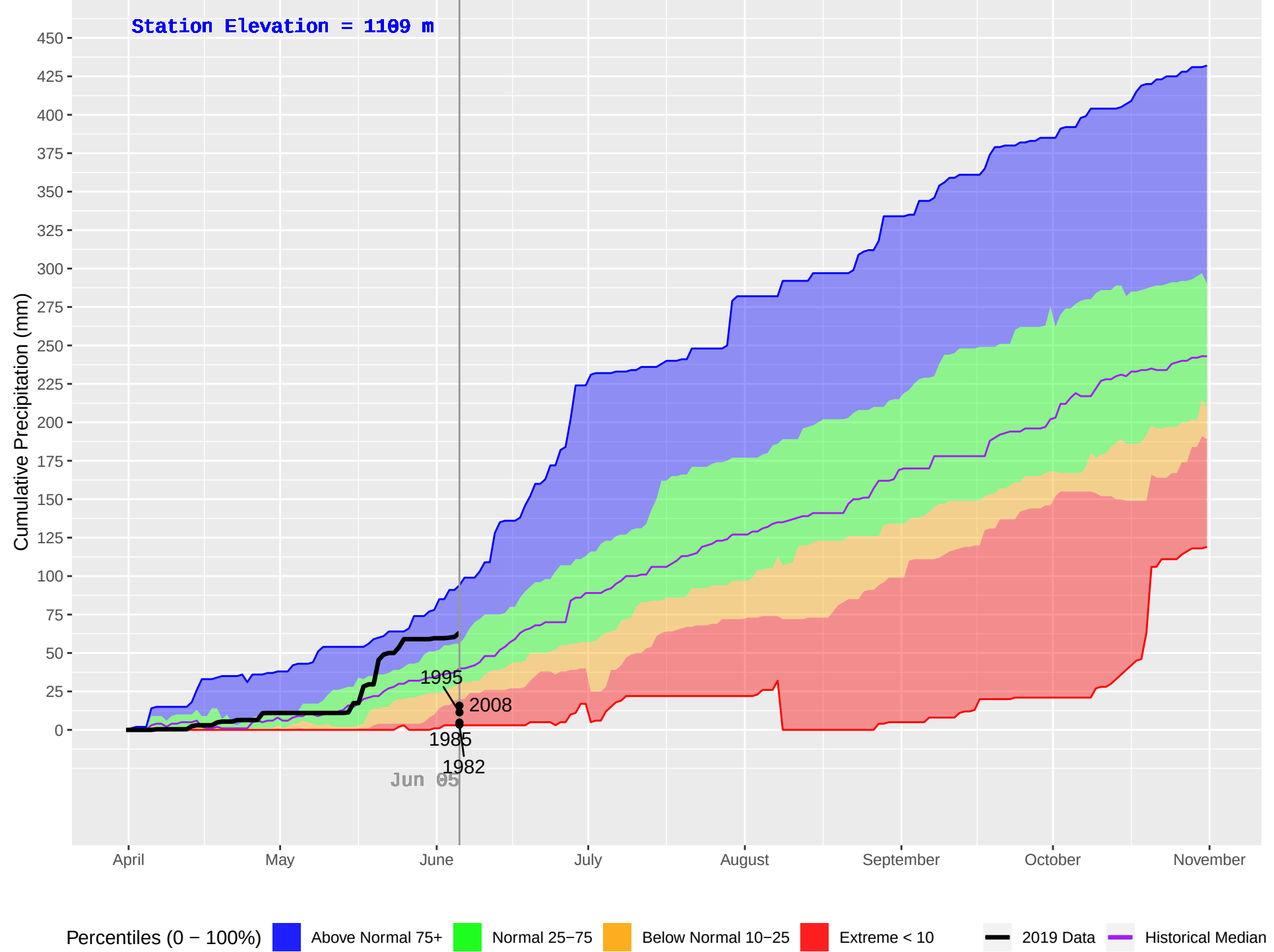
MOOSE LAKE (165) : Historical (1980–2018), Current (2019) Daily Cumulative Precipitation
