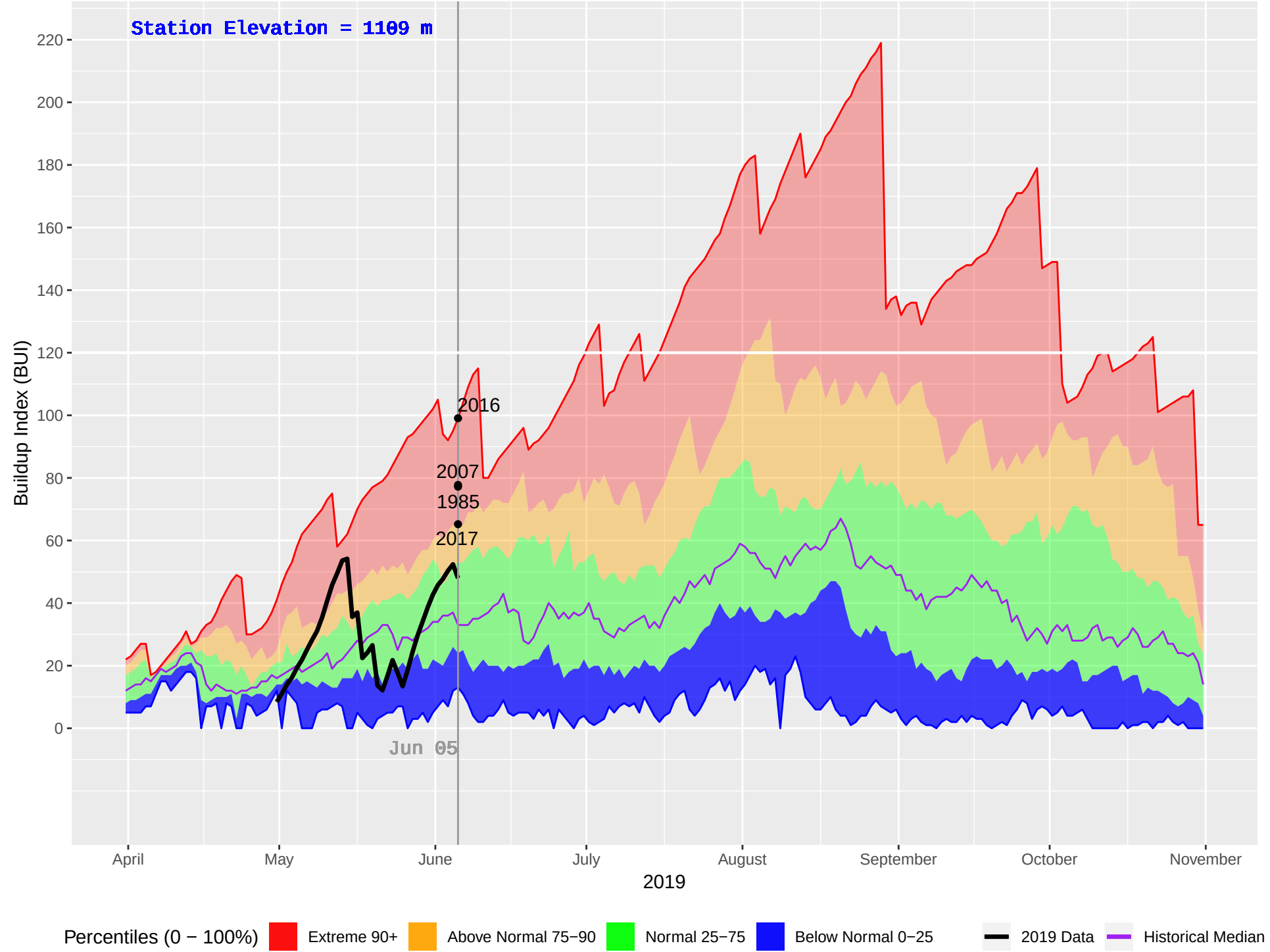
MOOSE LAKE (165) : Historical (1980–2018), Current (2019) Daily Buildup Index (BUI)
